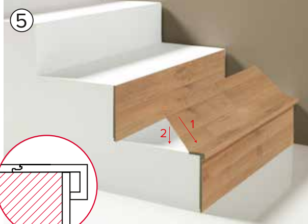
Place the floor plank anchoring it with the Loc system.
